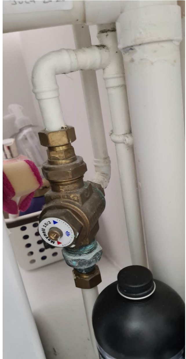
The Warren TMV
